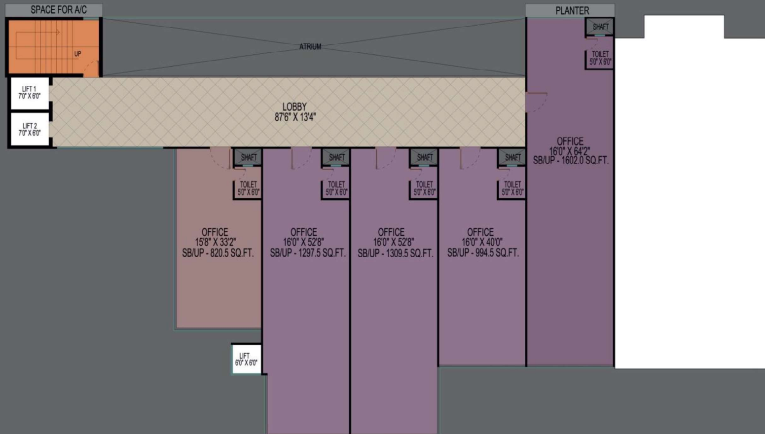
III FLOOR PLAN
